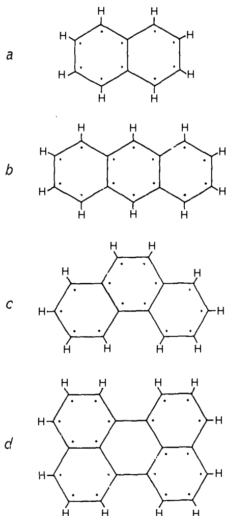
Fig. 8.6 The molecules of (a) naphthalene, (b) anthracene, (c) phenanthrene, and (d) perylene. Carbon atoms are at all corners and intersections in the diagrams.
