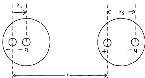
Fig. 4.3 In the coupled-oscillator model of two atoms interacting with the dispersion force, a portion of the negative charge cloud in each atom is instantaneously displaced from the nucleus, to give the atoms instantaneous dipole moments of magnitudes qx_1 and qx_2 .
