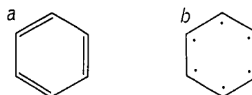
Fig. 8.13 The "resonance energy" of benzene is the difference between the energies of the molecule when six of its electrons are engaged (a) in localized and (b) in non-localized bonding.
