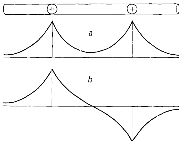
Fig. 6.1 For the delta-well model of the hydrogen molecule-ion in Chapter 5, the two one-electron wave functions are spacially symmetrical (a) and antisymmetrical (b).
