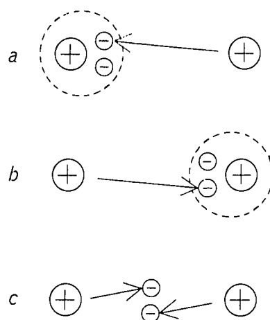
Fig. 2.2 Three formal arrangements of two electrons in a hydrogen molecule. When both electrons are near one or the other nucleus (a and b), there is a net negative charge within the dotted line, and the two atoms attract each other as two ions would. When the electrons are between the nuclei (c), they attract both nuclei toward them, and thus toward each other.
