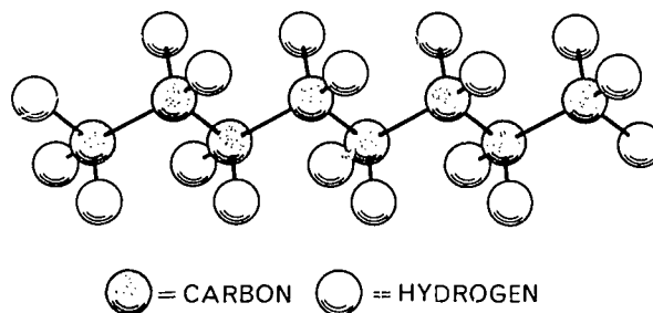
Fig. 9.1 The chain of carbon atoms in the hydrocarbon, n -octane ( C_8H_{18} ), linked by sp^3 bonds, exemplifies the simplest type of organic compounds. This and the succeeding diagrams of molecules are not drawn to scale. They are intended only to show the bonding connections between the atoms, and some of the spatial relations which those connections imply.
