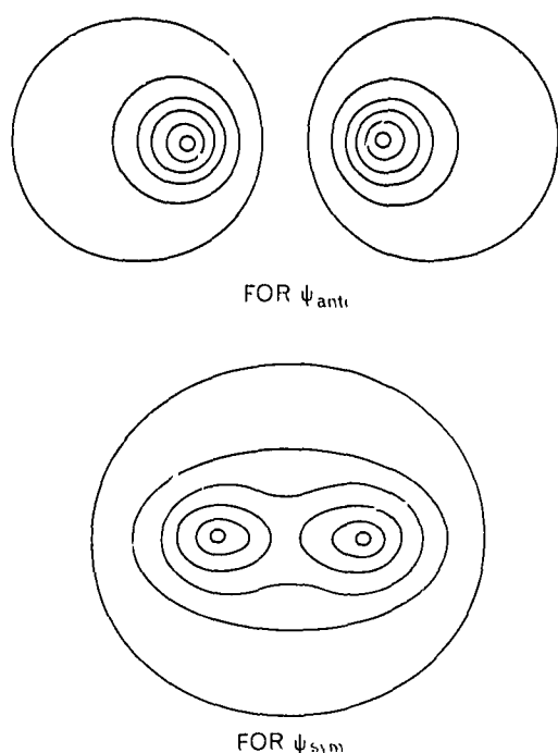
Fig. 6.6 Contours of equal electron density, in a plane containing the two nuclei, for the spatially antisymmetric and the spatially symmetric wave function for the hydrogen molecule in the approximation of Eq. (6.1).
