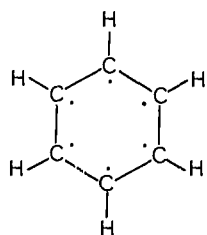
Fig. 8.4 The extended wave functions of the molecule of benzene must accommodate one electron from each carbon atom, left over after the other three electrons of principal quantum number 2 have been used to form localized bonds.
