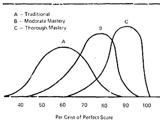
Figure 1. Distributions of Achievement Test Scores Under Traditional Treatment and Mastery Treatment (Hypothetical)
