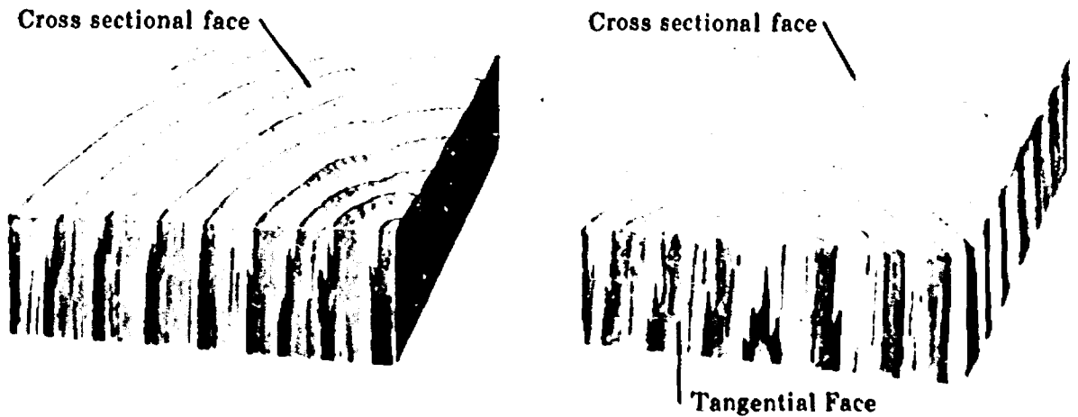
Figure 18.—For the specific gravity and shrinkage experiment, the wood blocks must be cut so that the growth rings appear as in specimen at top right, and not as in top left. Lower illustration shows a dial gage with a specimen in place.
