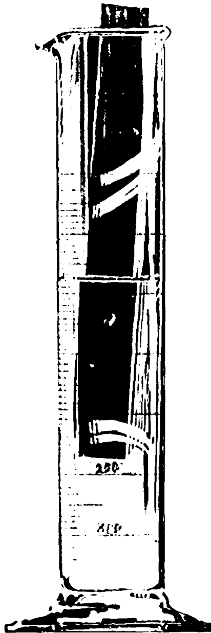
M-134,259 Figure 17.—A tall glass cylinder is necessary for the specific gravity test, so that the block will float almost upright, giving a water mark at approximately a right angle to the length of the specimen.
