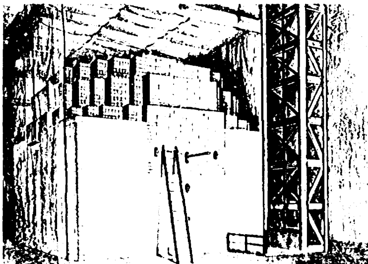
Sketch of the first pile. Around it is a tent of balloon cloth fabric, prepared so that the reactor could be sealed to minimize nonproductive loss of neutrons if necessary; the tent was never used. This is one of two drawings made in 1946 and based on physical measurements of the reactor and recollections of the scientists. (The other drawing is on page 33.)
