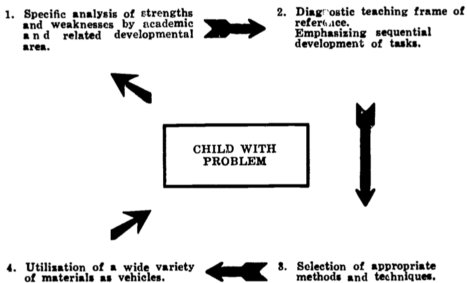
Diagram 1: General Approach
