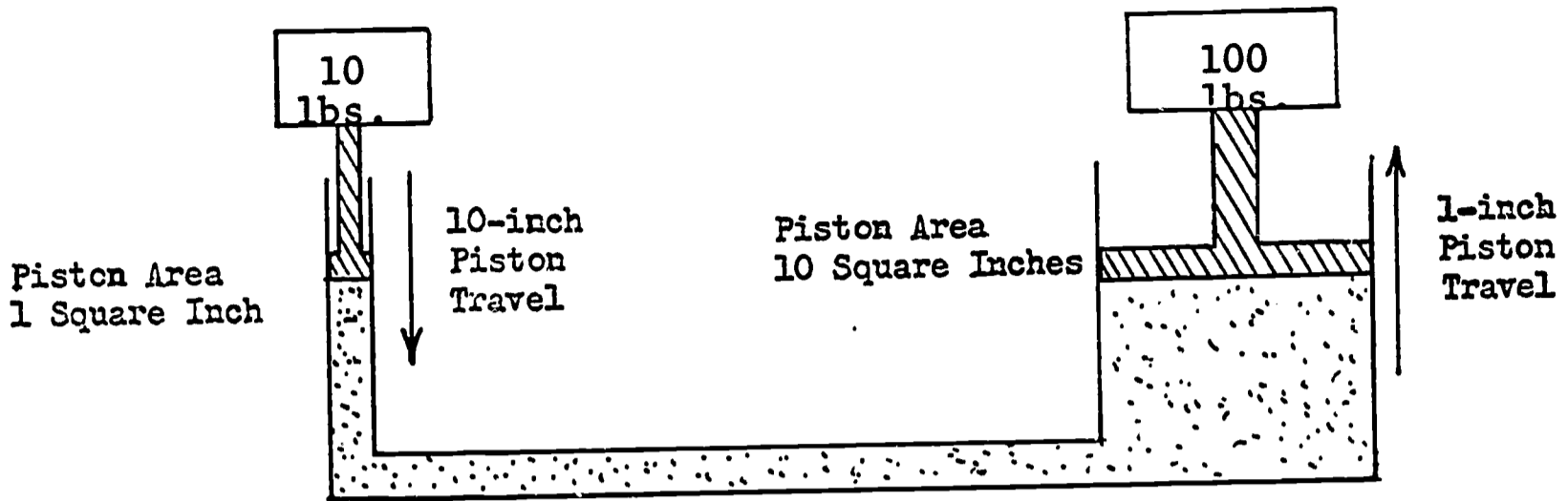
Figure 3. Hydraulic cylinder and differential area principles.
