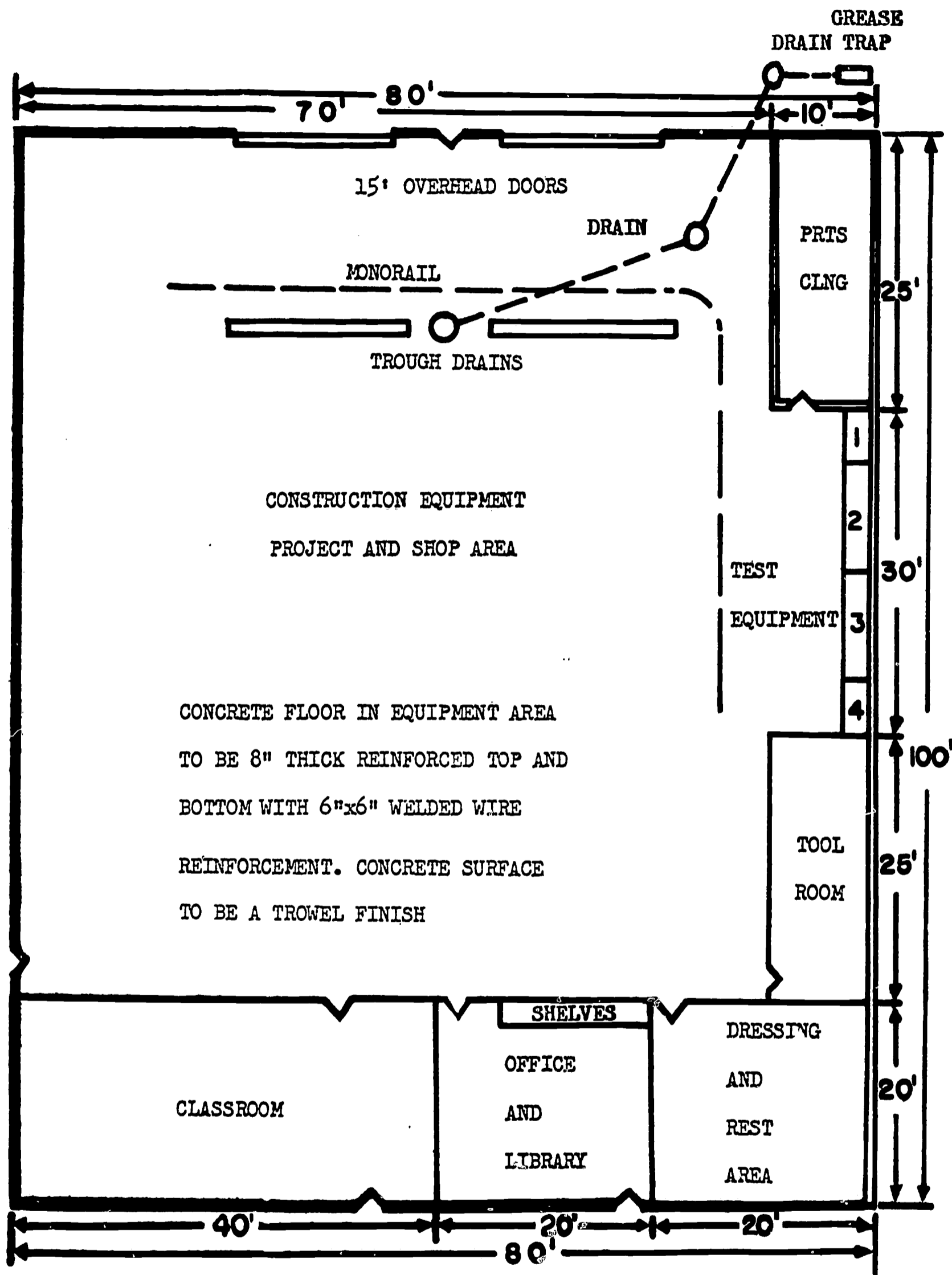
Figure 8. Suggested training facility.
