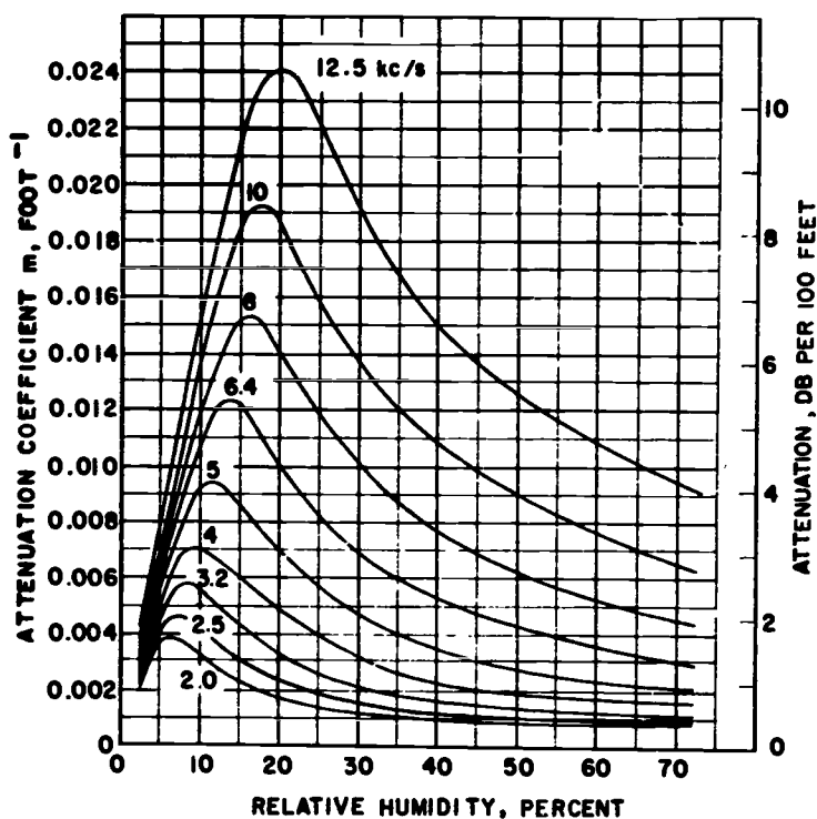
Figure 4 Effect of relative humidity on air absorption of sound at different frequencies. (Reproduced with permission from "Absorption of Sound in Air in the Audio-Frequency Range", Journal, Acoustical Society of America, Vol. 35, January 1963.
