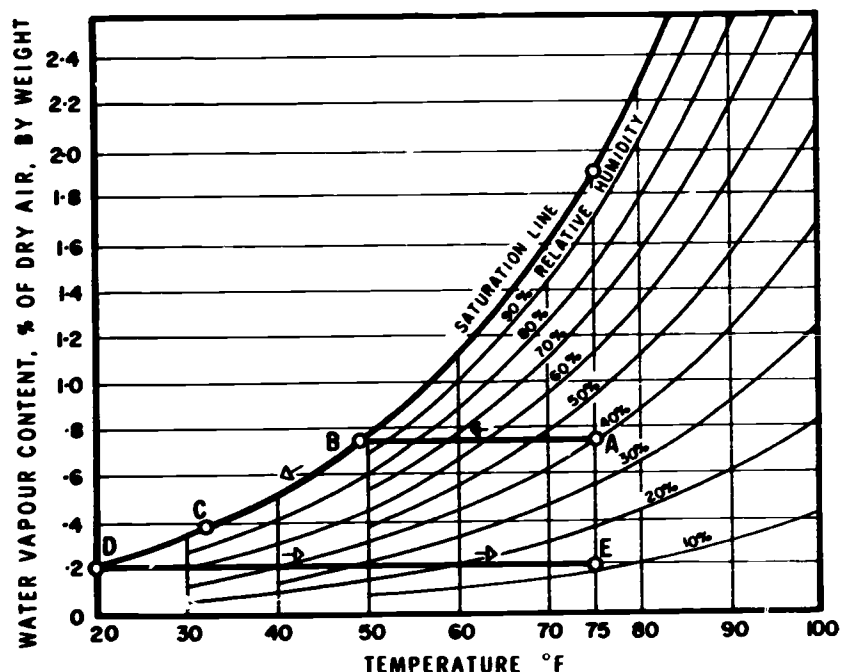
Figure 2 Simplified psychrometric chart showing properties and processes of air and water vapour mixtures.
