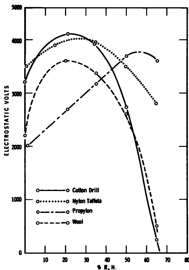
Figure 3 Electrostatic charging on fabrics at different relative humidities.
