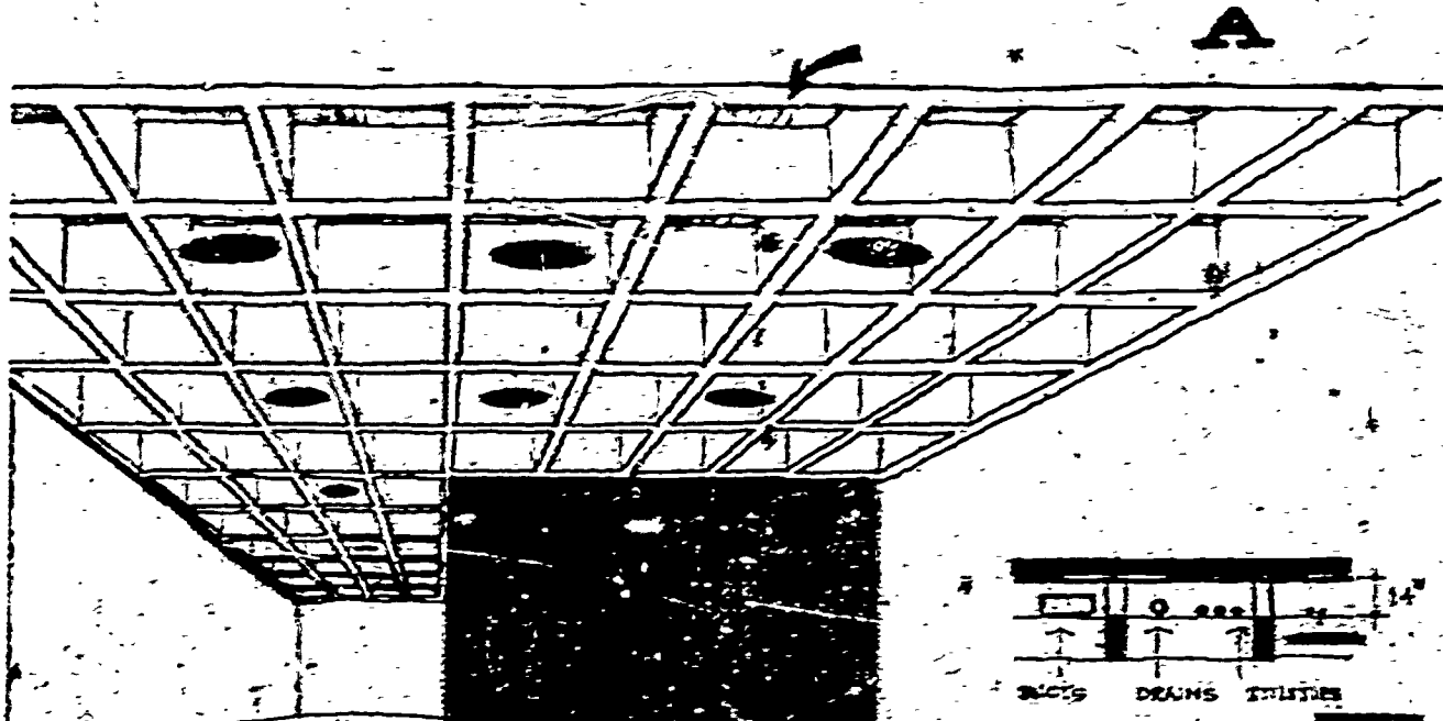
STRUCTURAL EGG-CRATE SEPARATED FROM FLOOR PROVIDES SCREENING AND SPACE FOR UTILITIES
