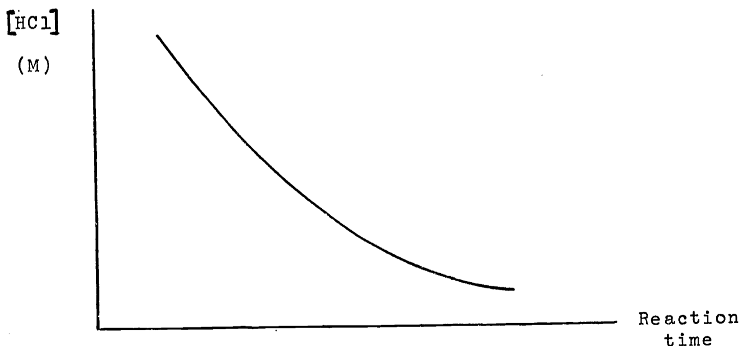
Fig. 1 Variation of reaction time with acid concentration.
