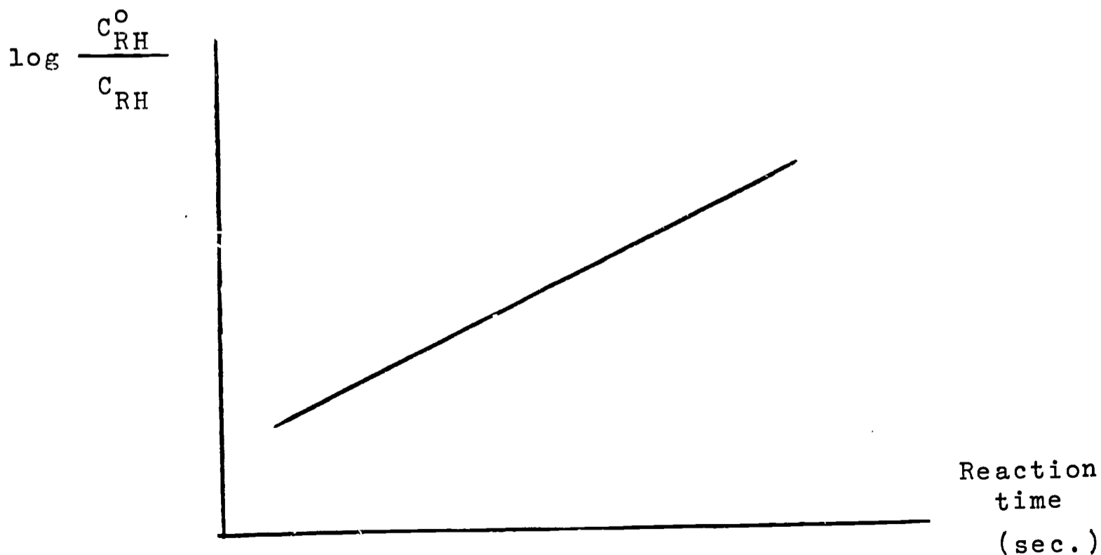
Fig.1. First order plot for hydrolysis of t -butyl chloride.
