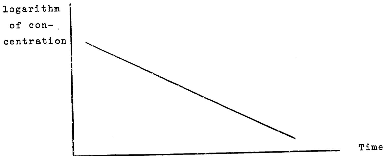
Fig.2 A plot of log c vs t time
