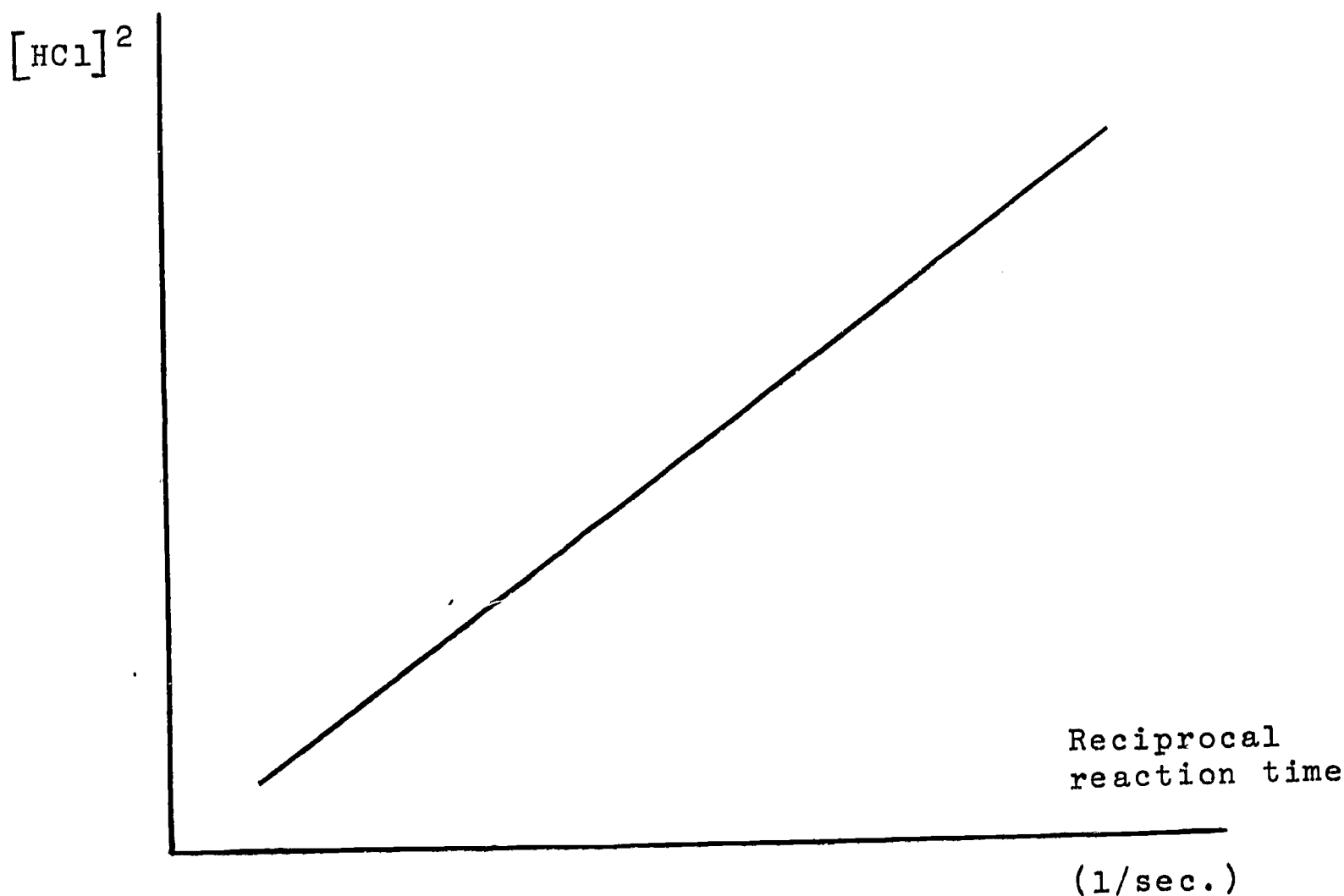
Fig. 2. Square of acid concentration against reciprocal reaction time ( \propto average rate of reaction).
