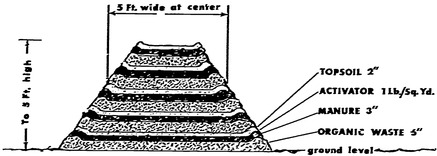
END VIEW OF TYPICAL COMPOST PILE
