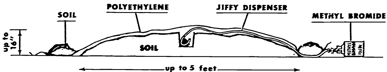
SOIL FUMIGATION WITH METHYL BROMIDE
