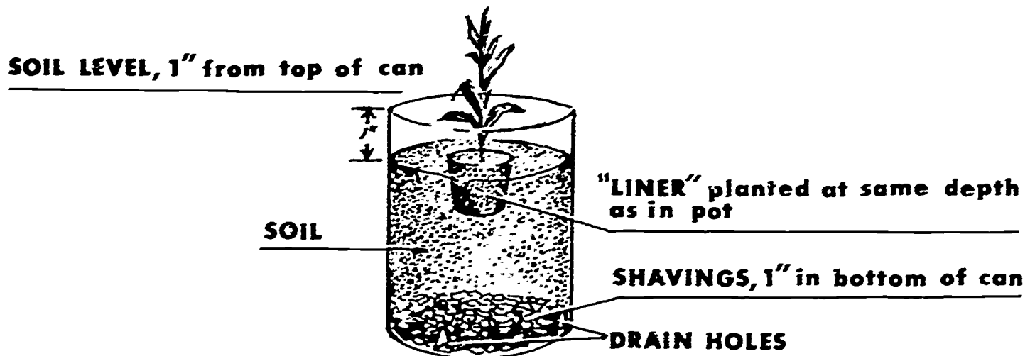
A PROPERLY CANNED PLANT
