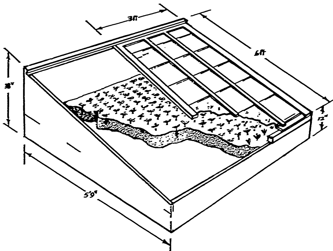
TYPICAL COMMERCIAL COLDFRAME
