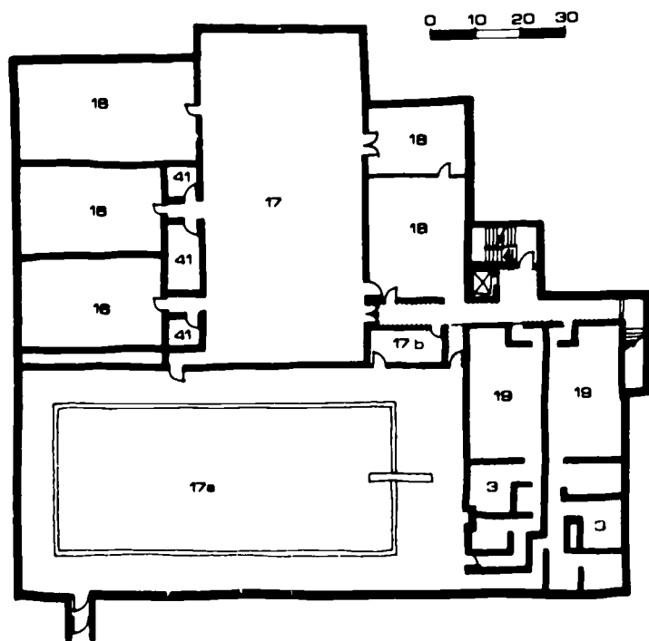
LOWER BASEMENT PLAN
