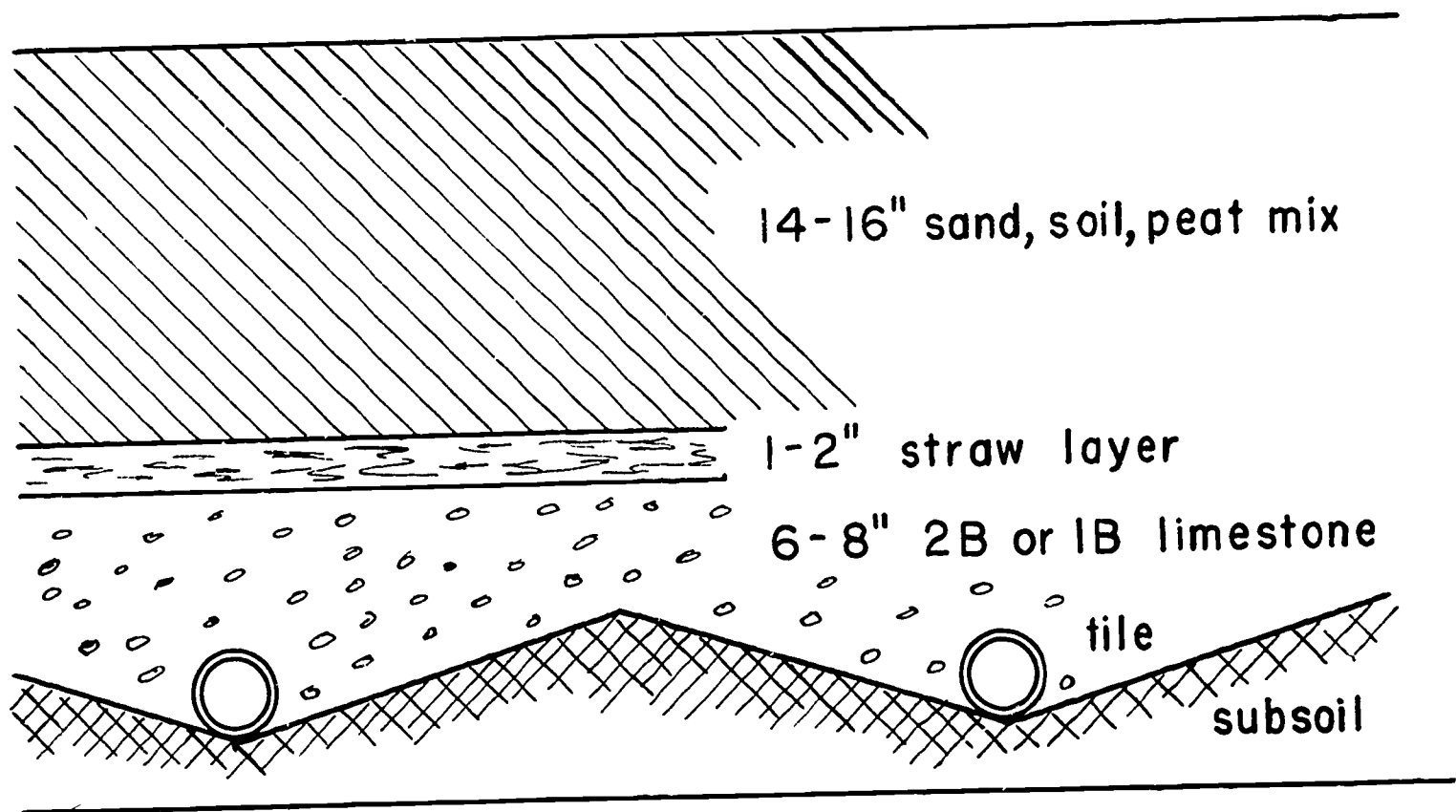
Figure 16. Cross-section of a golf green showing the drainage and construction materials. Tiles are placed in swales and covered with crushed stones.
