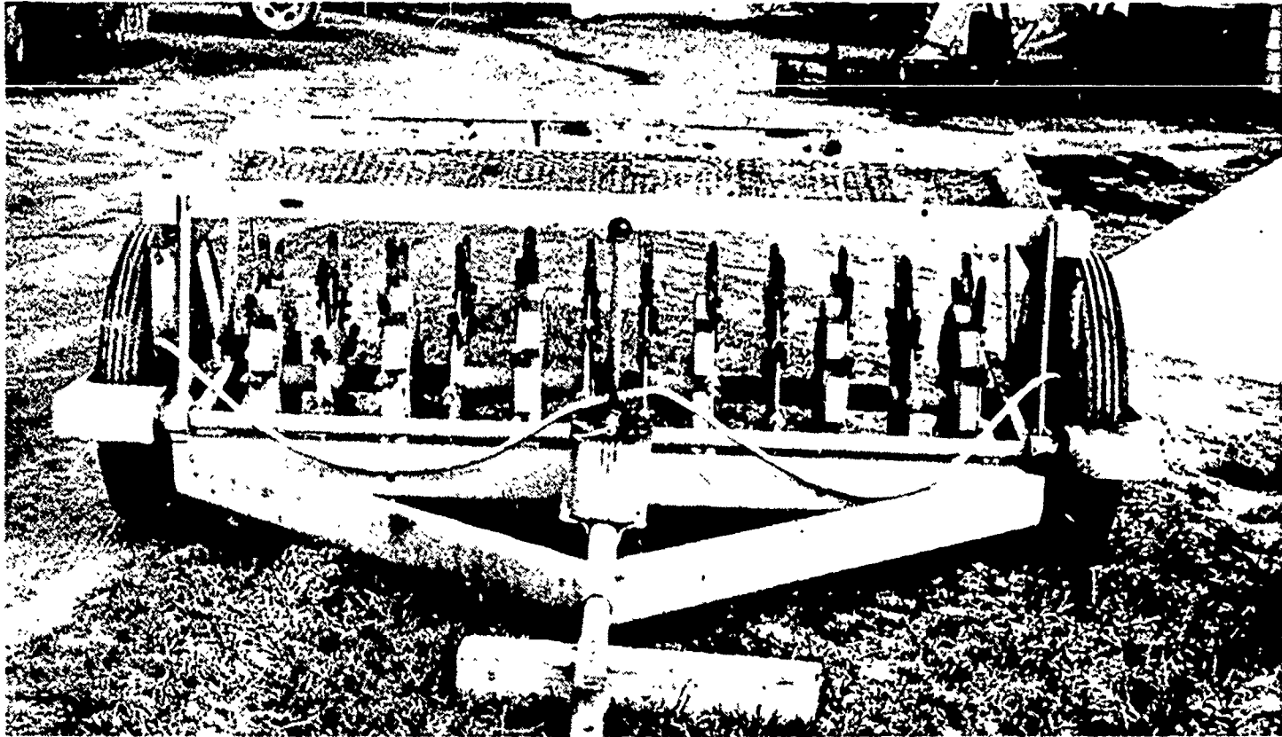
Figure 8. Tractor-drawn aerators are used to reduce soil compaction on athletic fields.
