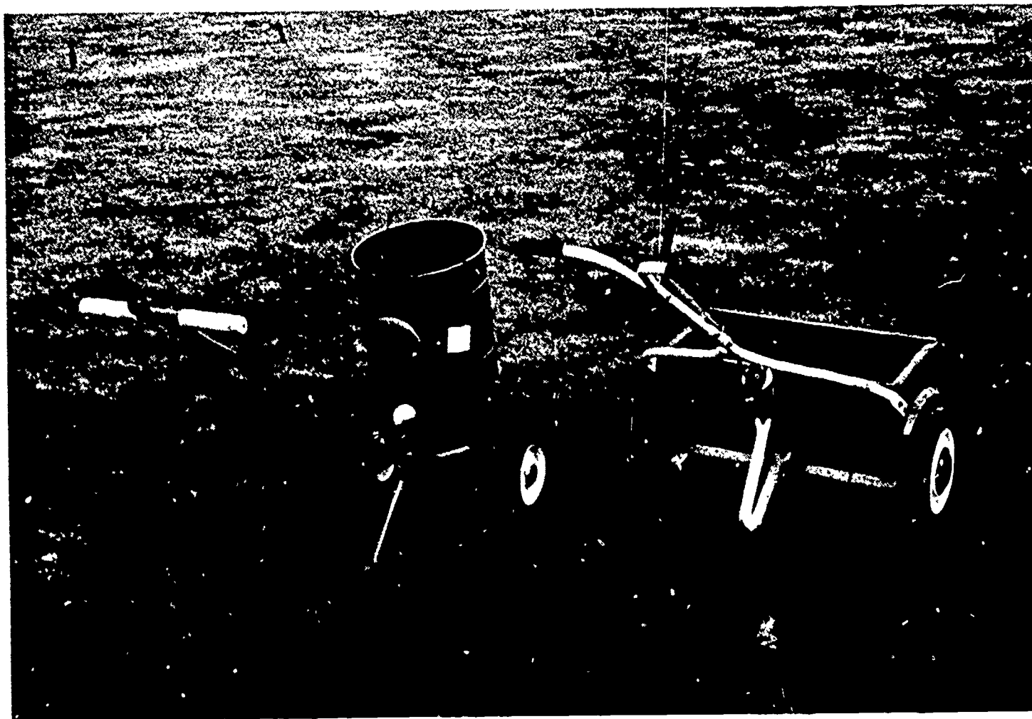
Figure 23. The broadcast seeder-spreader, left, and hopper seeder-spreader, right, may be used for sowing seeds (or for spreading fertilizer).
