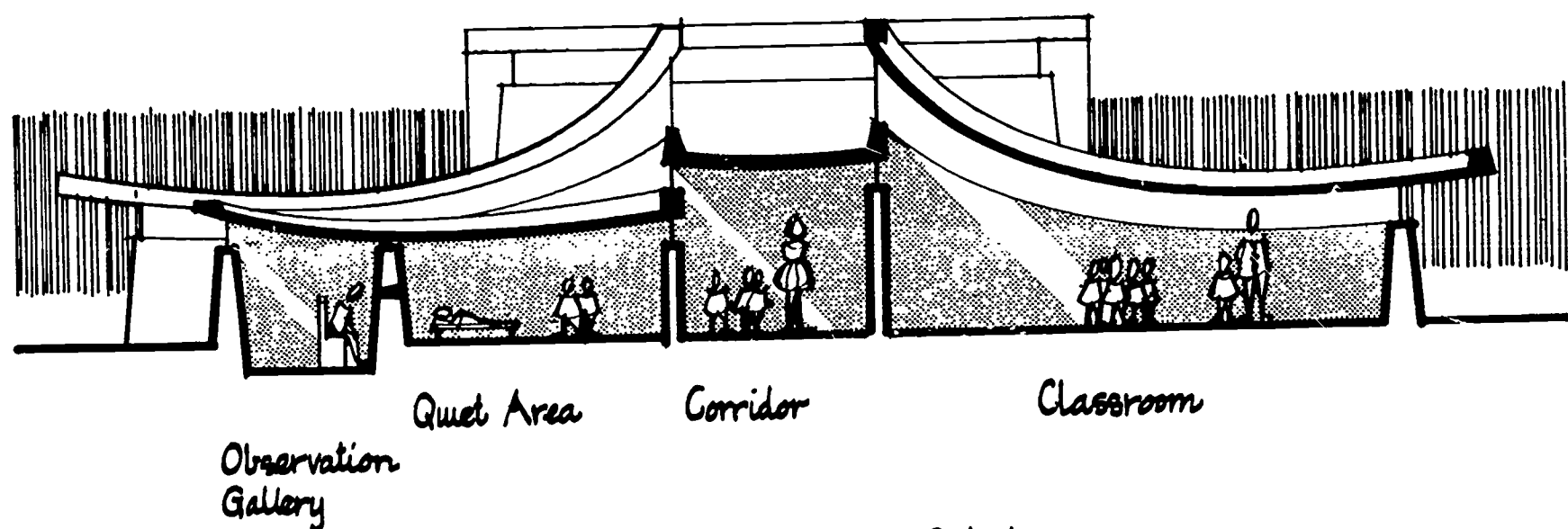
Typical Section through School
