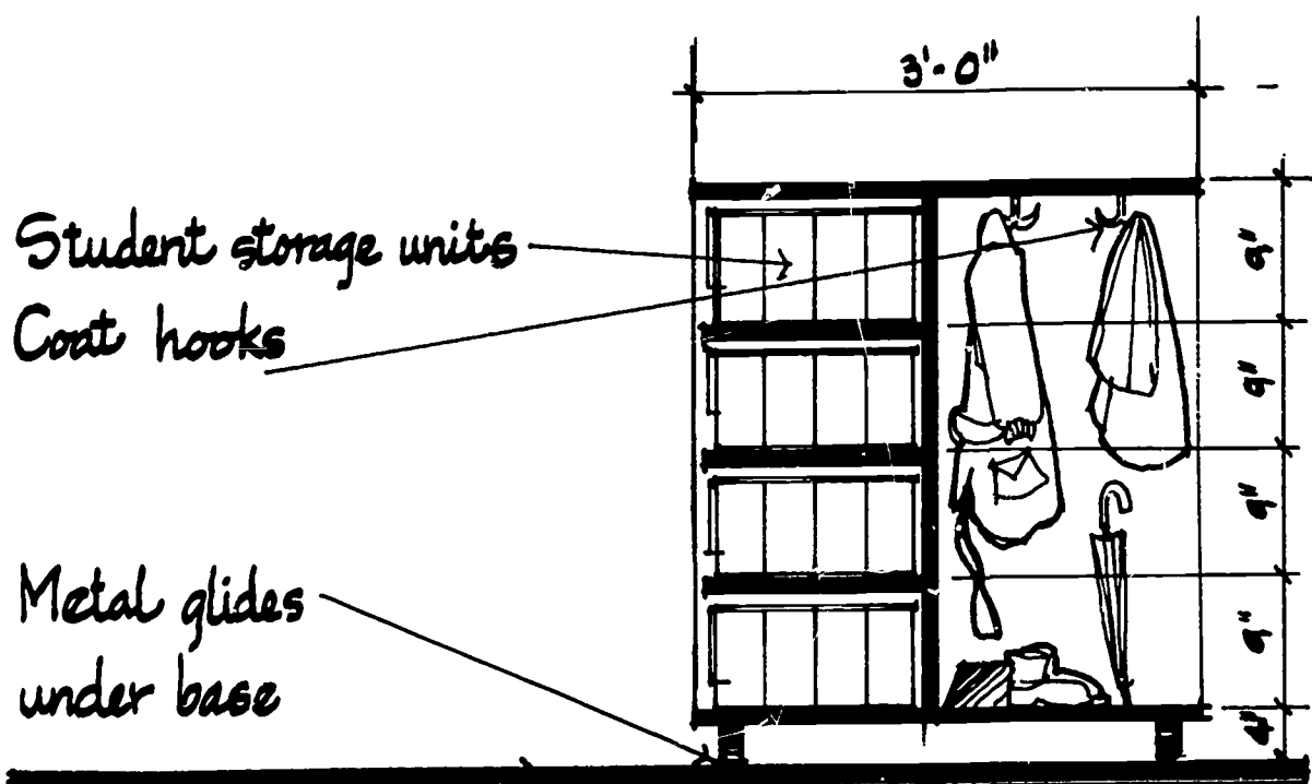
Section through storage unit
