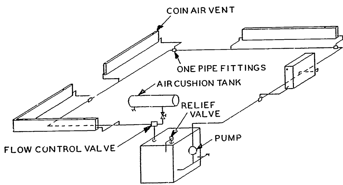
Schematic one-pipe forced hot water system (closed system)
