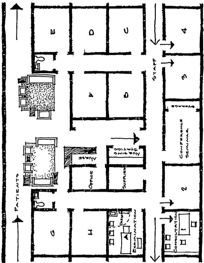
FIG. 18 PLAN OF SCHEME B
