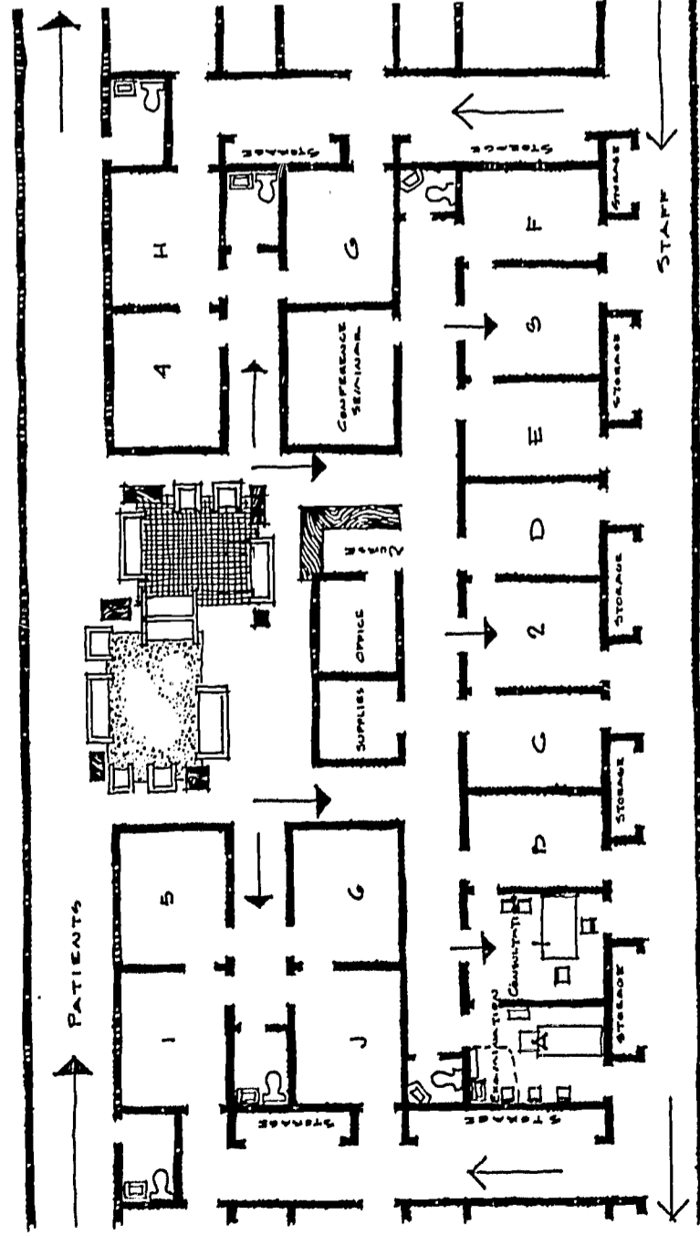
FIG. 18 PLAN OF SCHEME E
