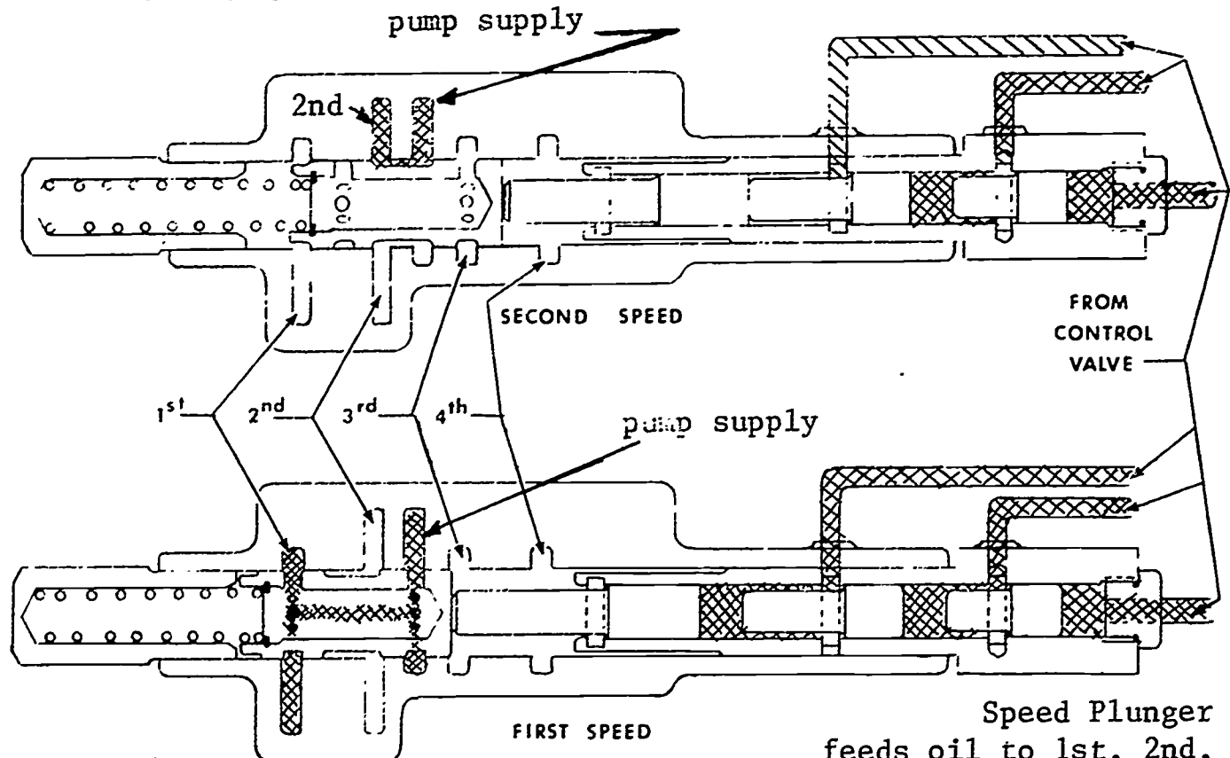
Fig. 14 Range valve and speed valve in different positions
