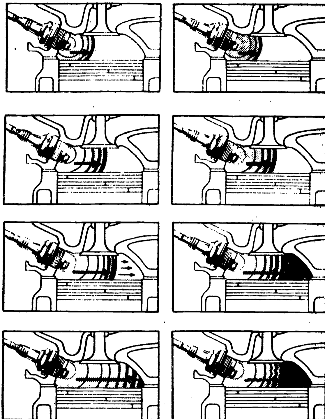
Fig. 12 Flame movement
