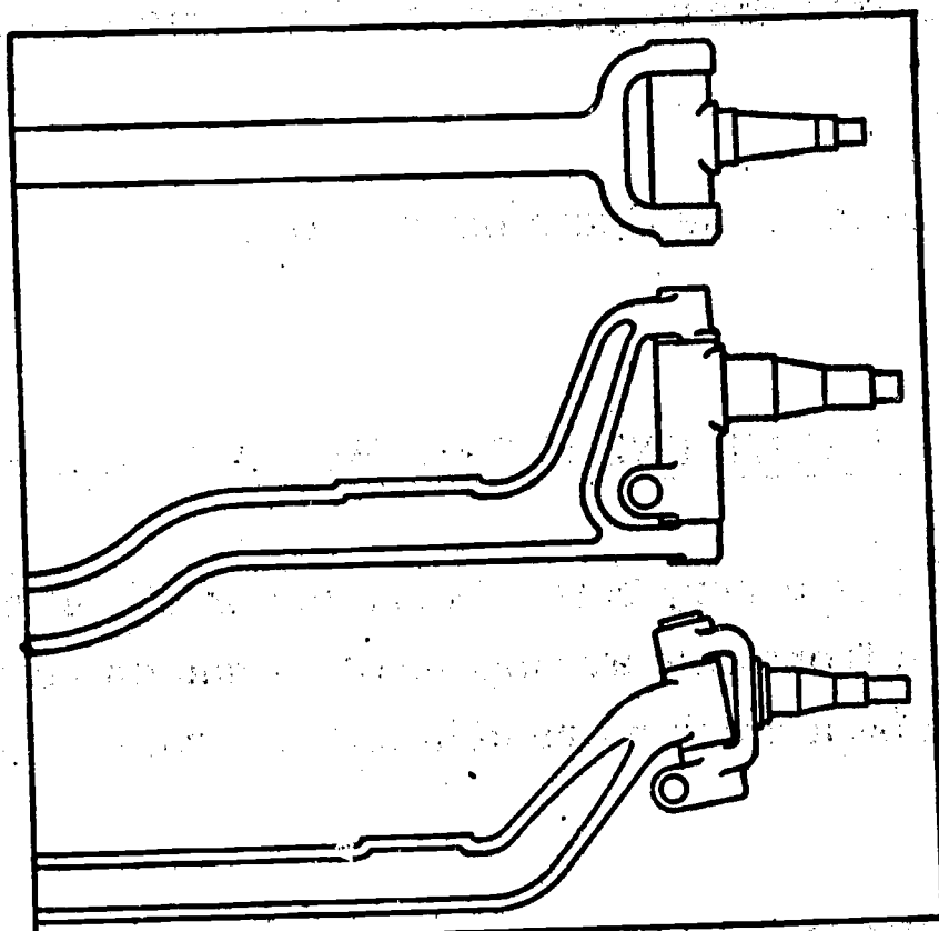
Fig. 5 Three front-axle types.
