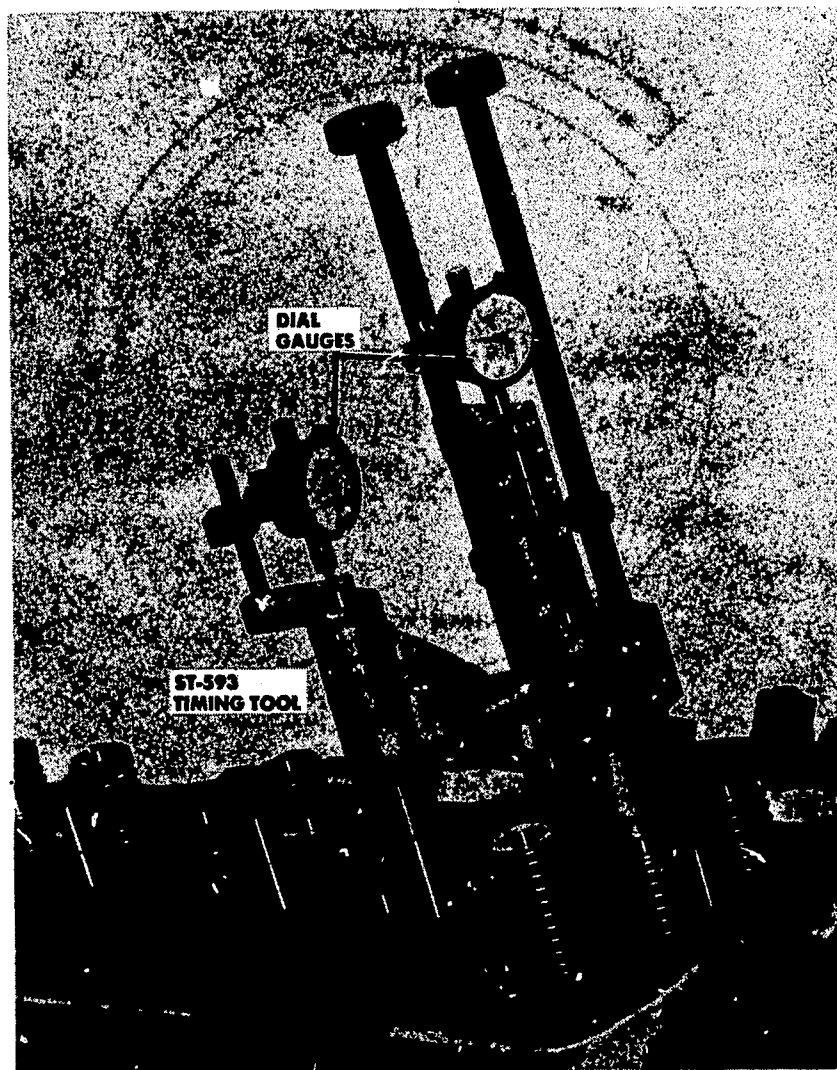
Fig. 1 . ST-593 injector timing fixture.
