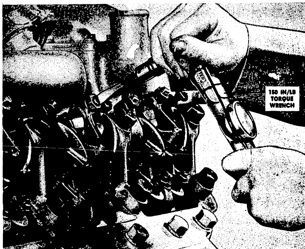
Plate II Adjusting injector.
