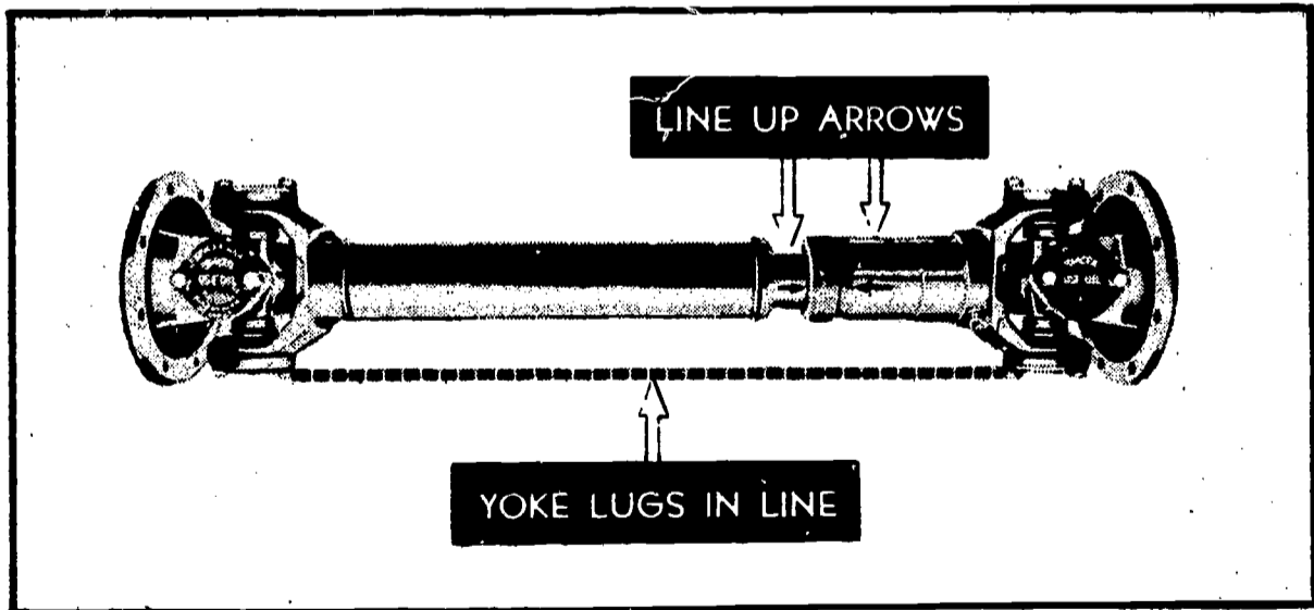
Fig. 16 Assembled drive line.
