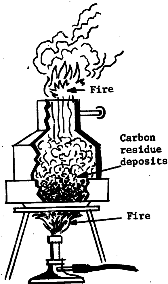
Fig. 11 Conradson test.
