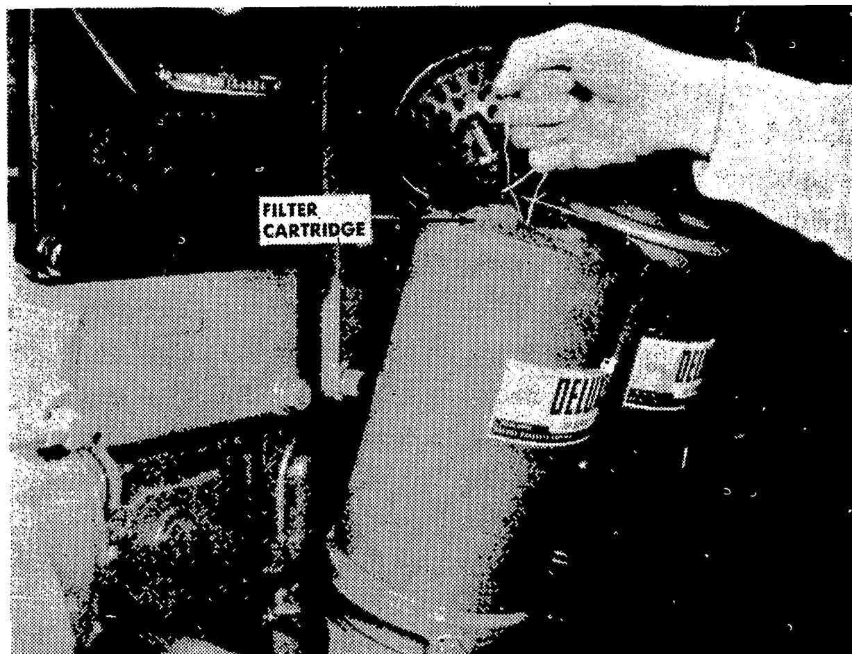
Fig. 7 Twin by-pass filter unit.
