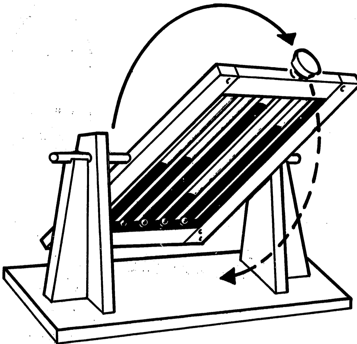
Fig. 12 Testing for oil viscosity.
