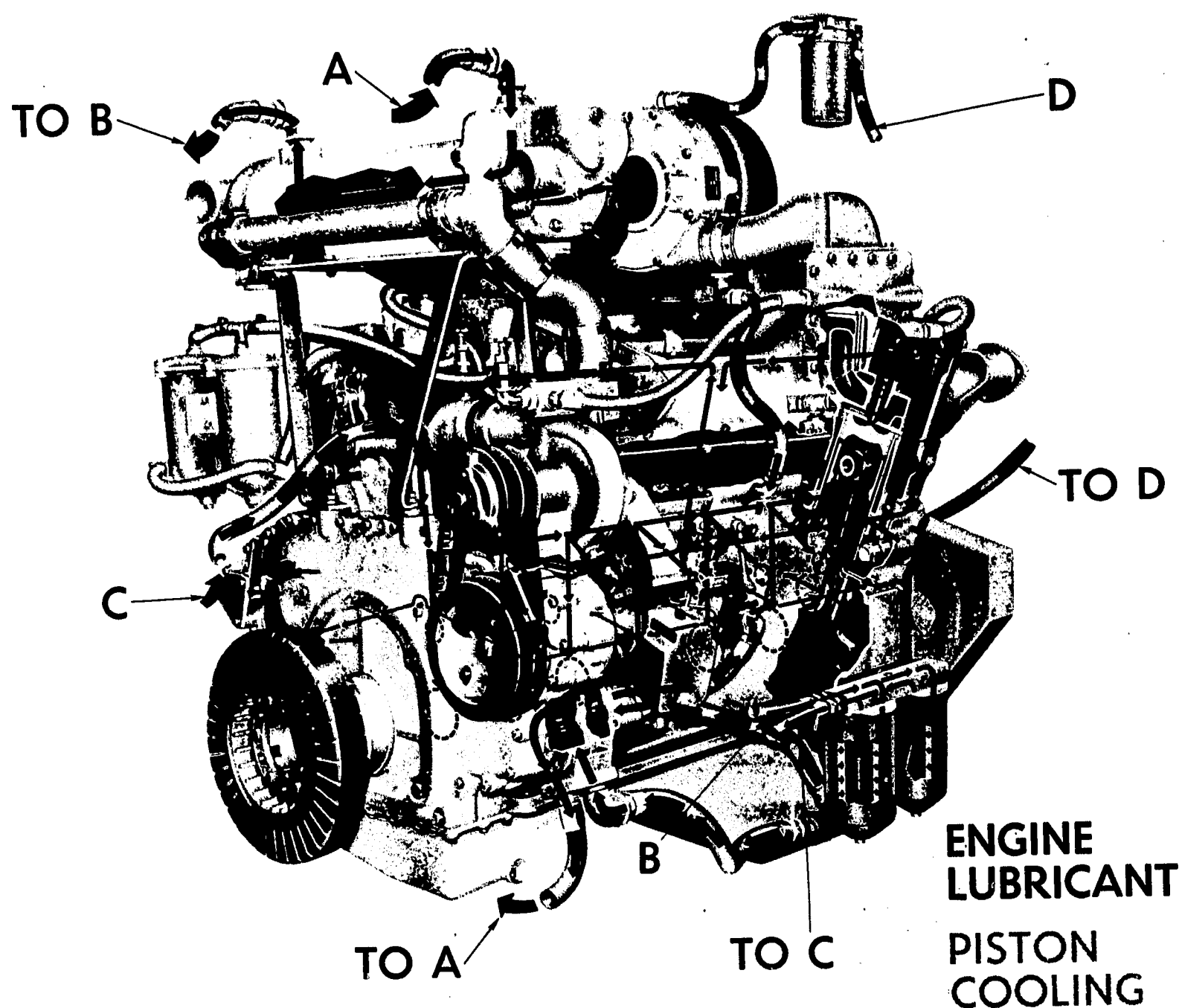
Fig. 4 Lubricating oil flow VT12-700.
