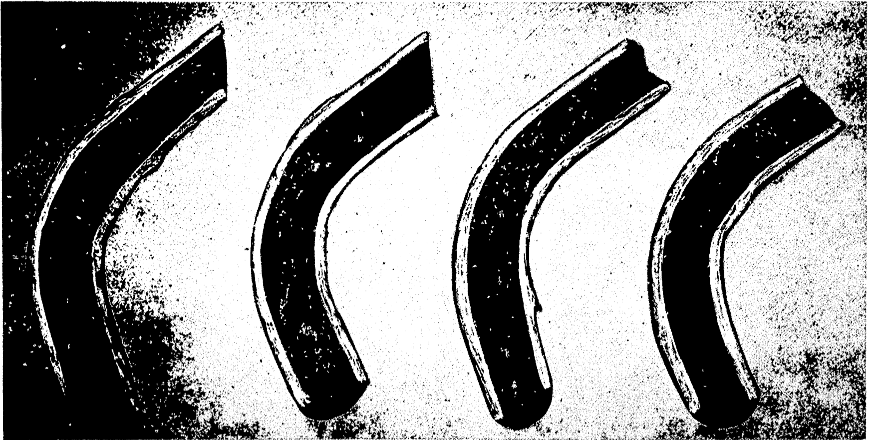
Plate I Half sections of an oil line that have become plugged with the coffee ground type of deposit.
