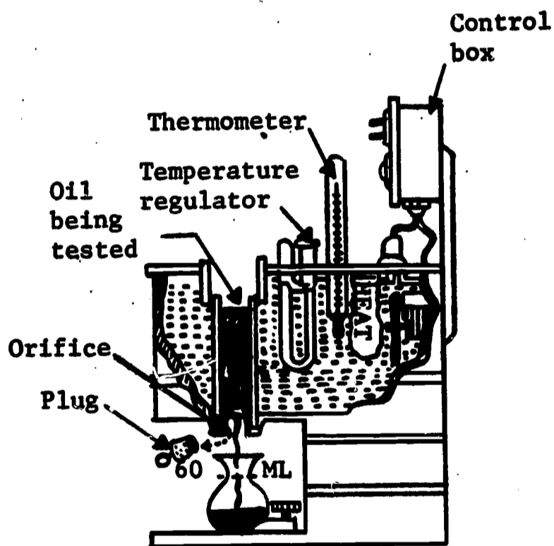
Fig. 8 Saybolt viscosimeter.
