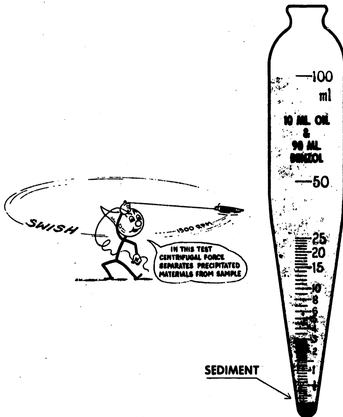
Fig. 13 Sediment test.
