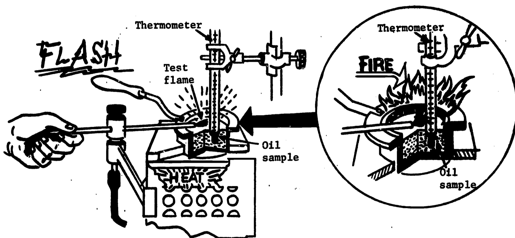
Fig. 9 Testing for flash and fire points.
