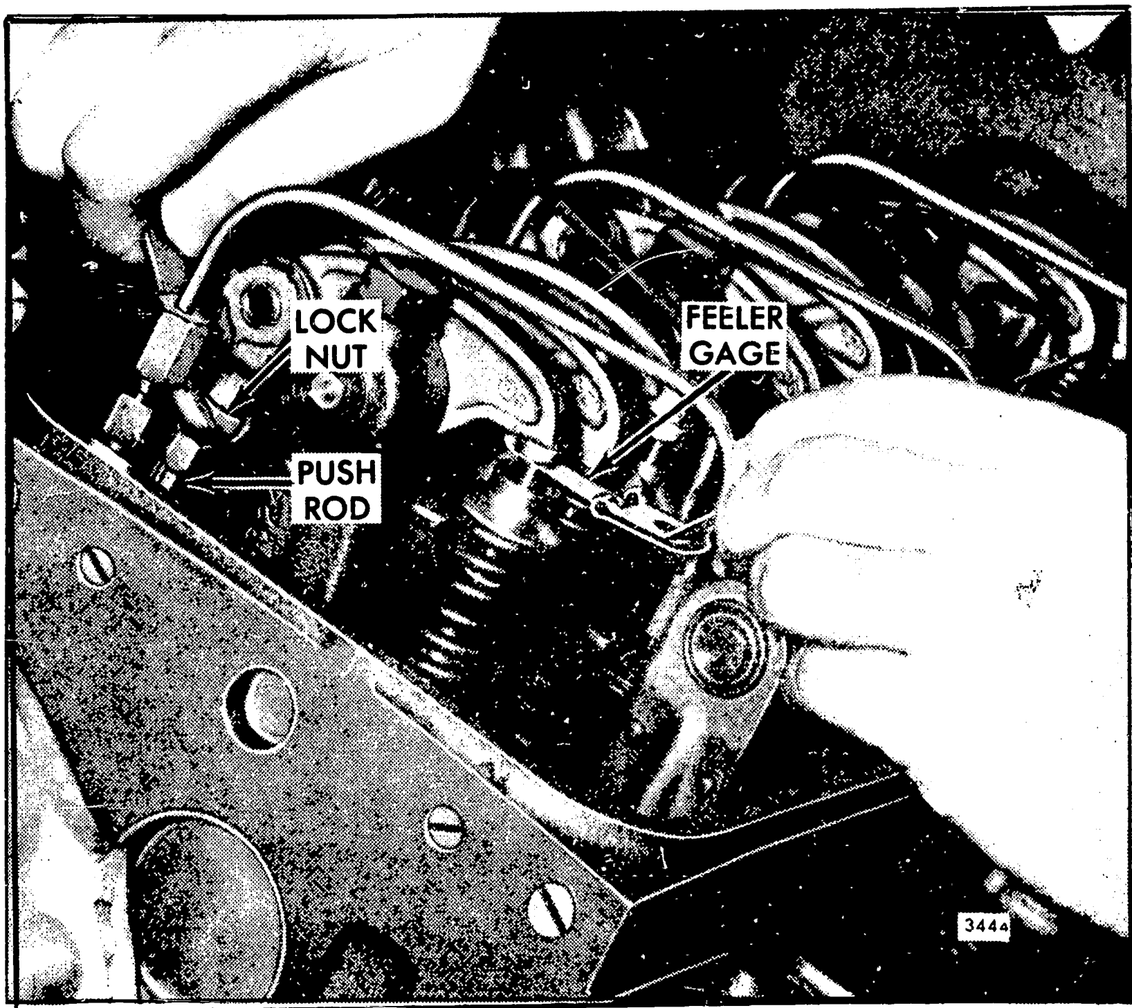
Plate I -- Adjusting valve clearance.
