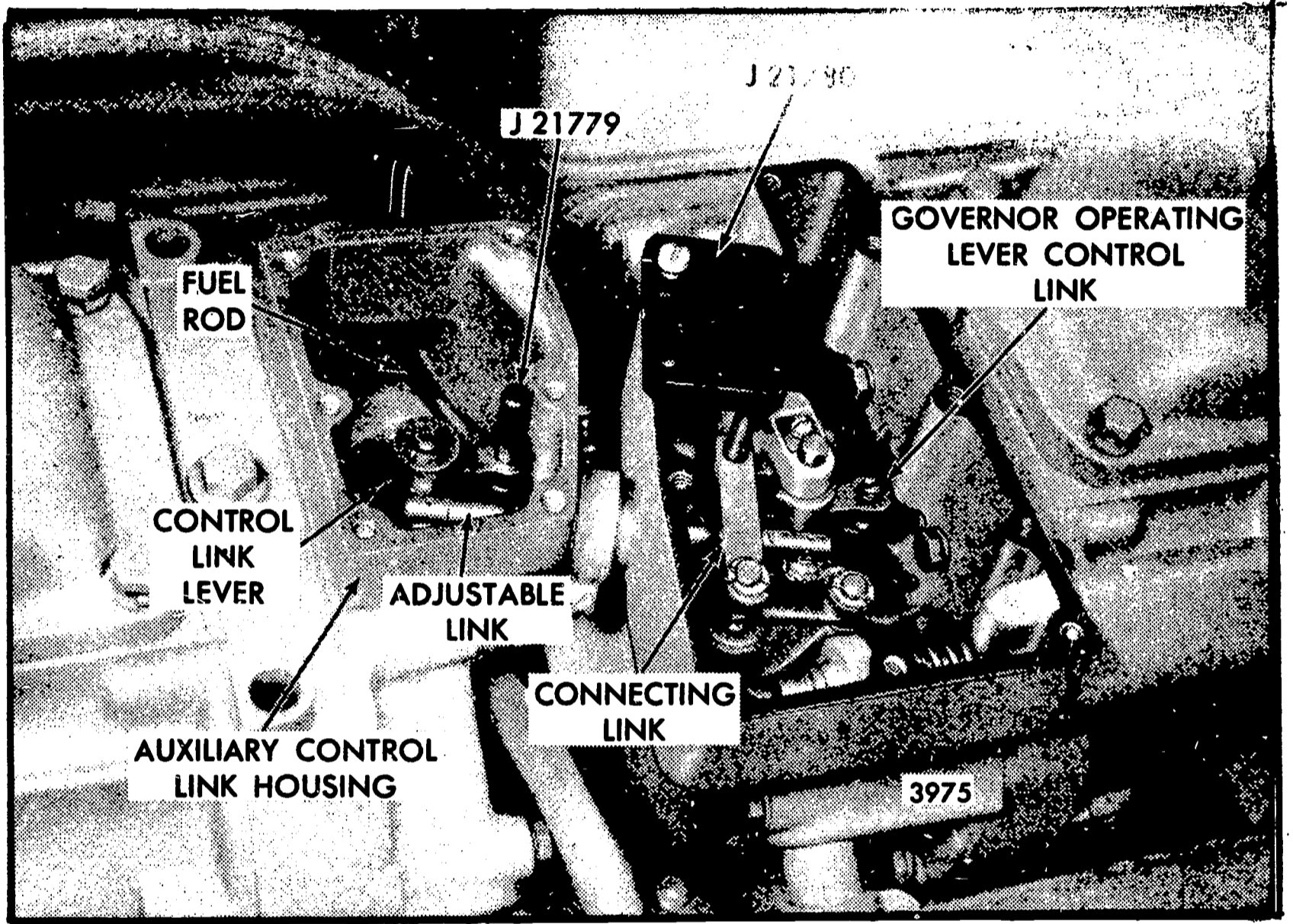
Plate III -- Positioning control link levers.
