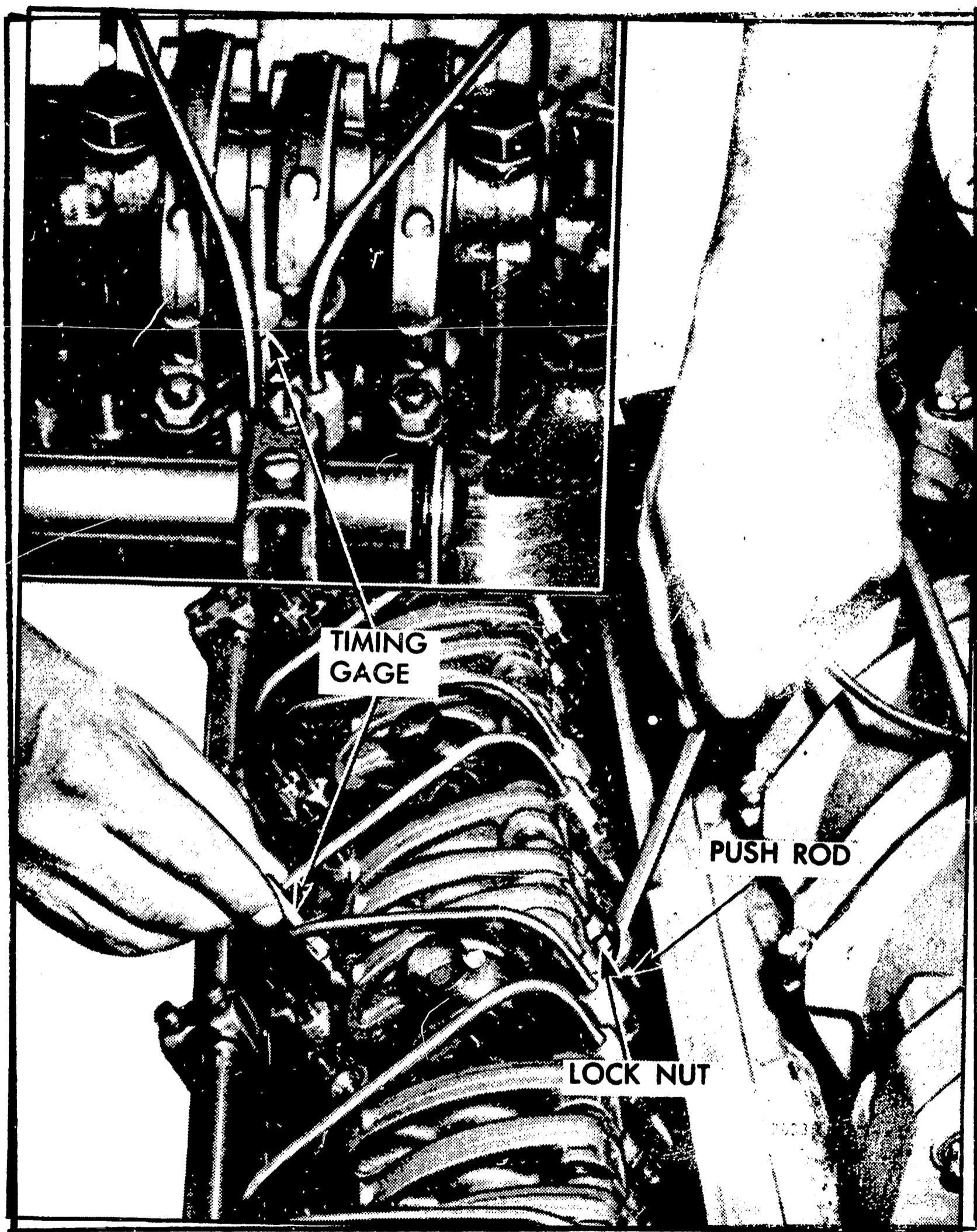
Plate II -- Timing fuel injector.
