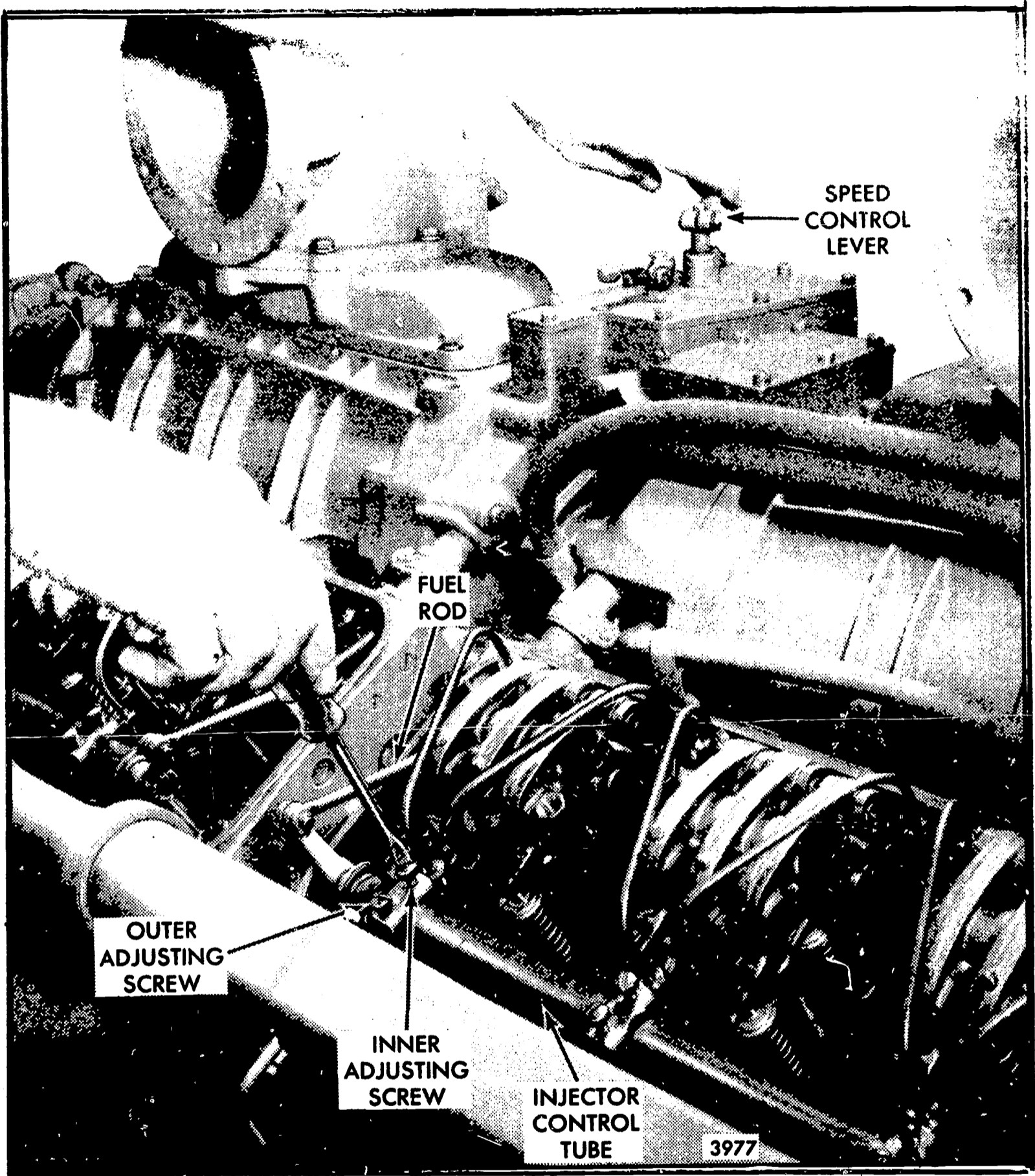
Plate V -- Positioning No. 4R injector rack control lever.
