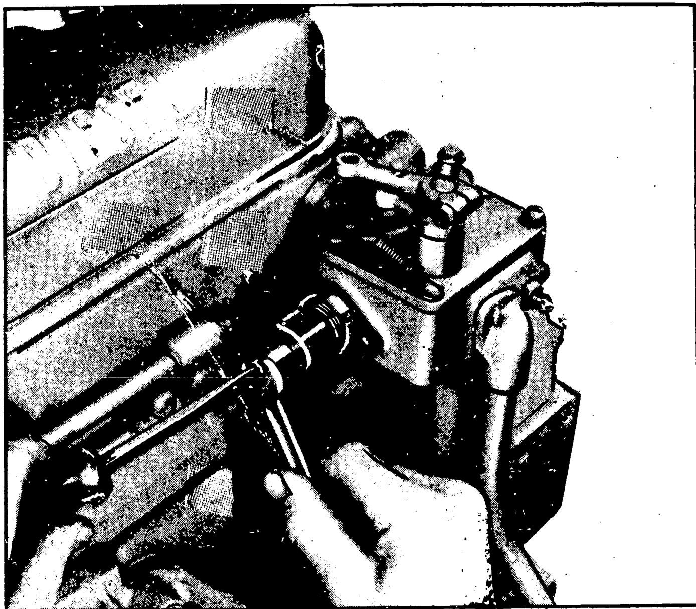
Fig. 6 - Adjusting idle speed.
