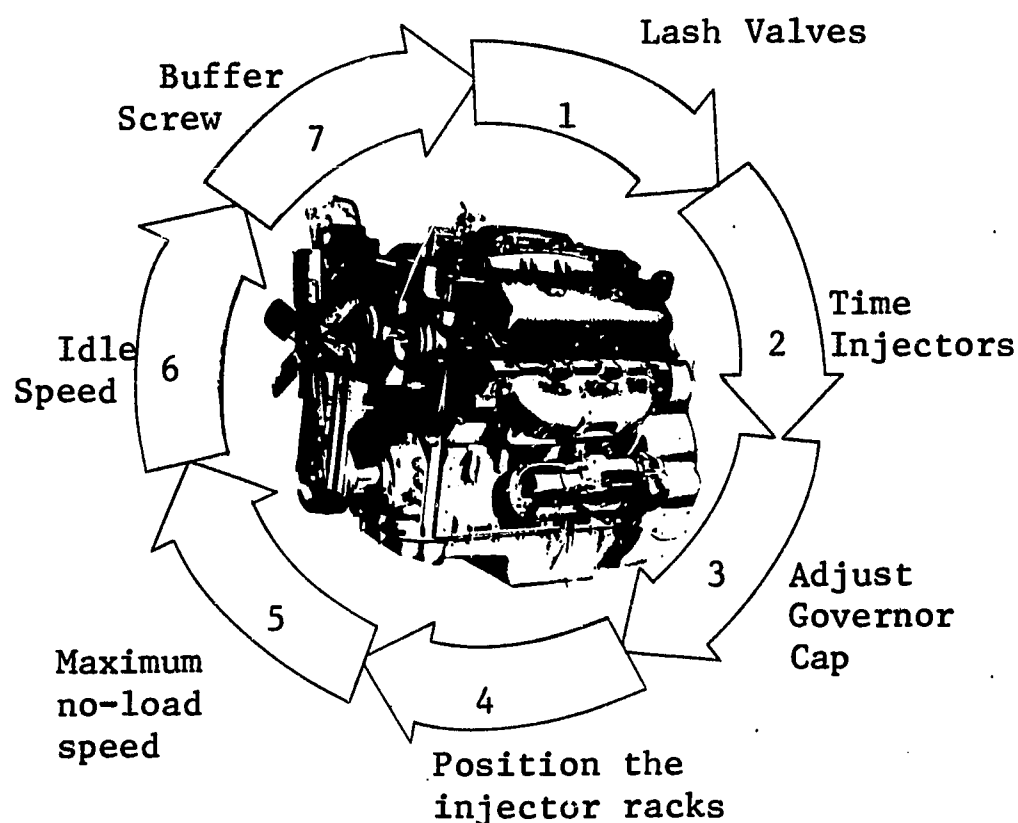
Fig. 15 - Summarizing engine tune-up.
