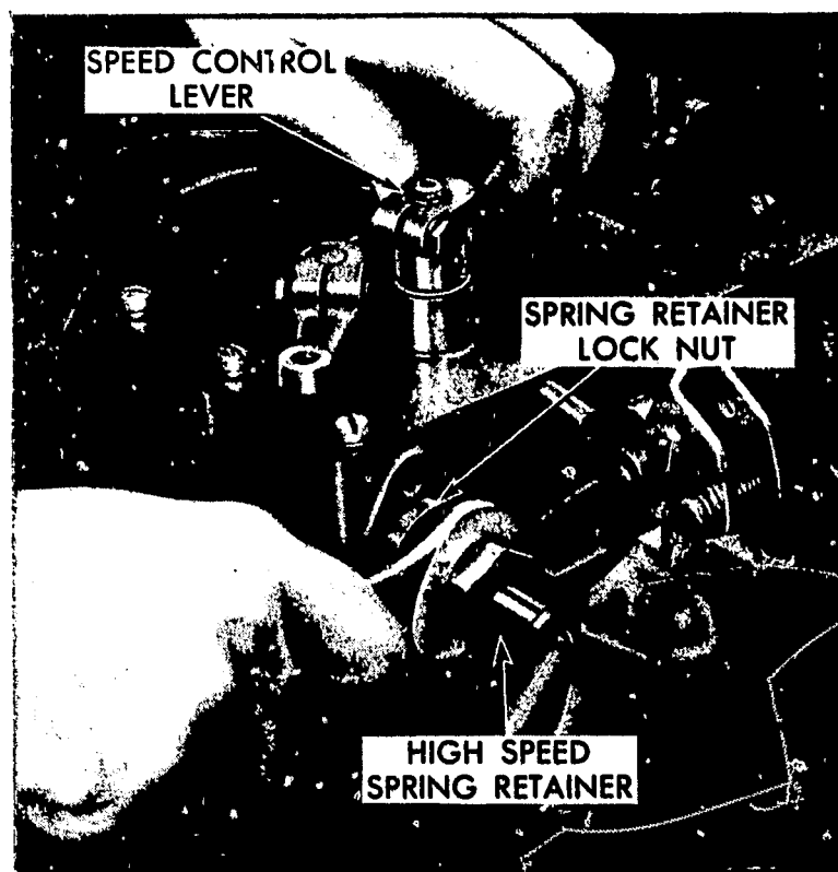
Fig. 11 - Adjusting Maximum No-Load Speed
