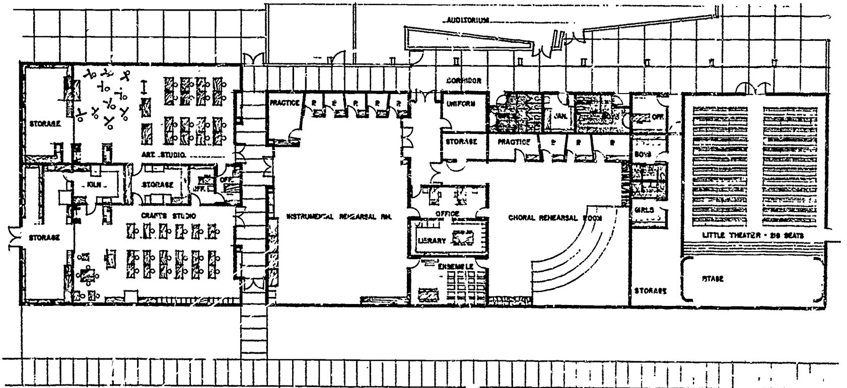
The specialized nature of music activities requires appropriate facilities necessary. Henry D. Sheldon High School, Eugene, Oregon Lutes and Amundson, Architects
