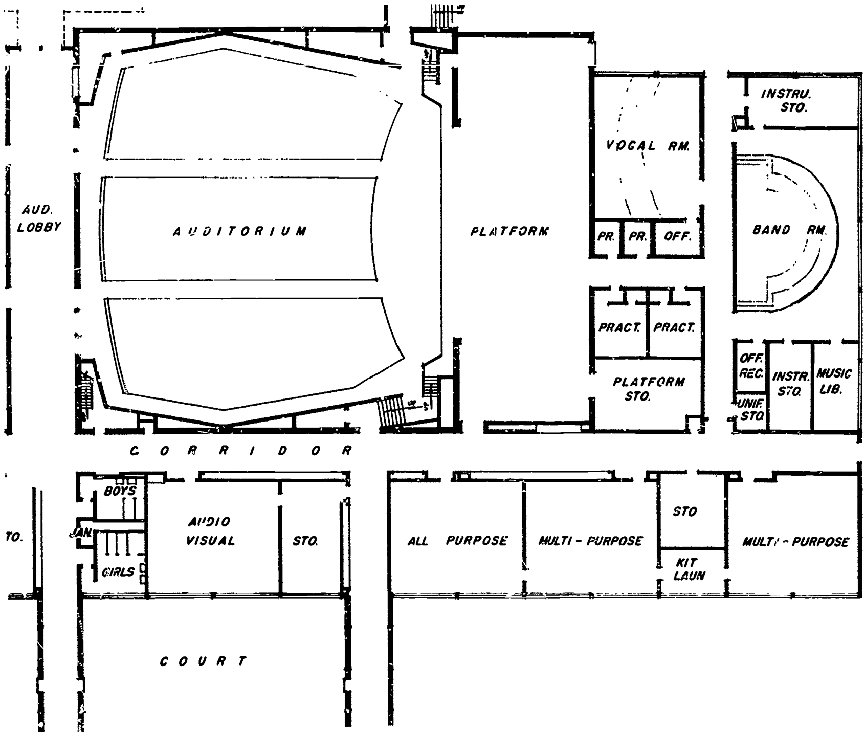
Easy access from the instrumental rehearsal room to the stage is highly desirable. Hanover (Pennsylvania) High School Hunter, Campbell & Rea, Architects
