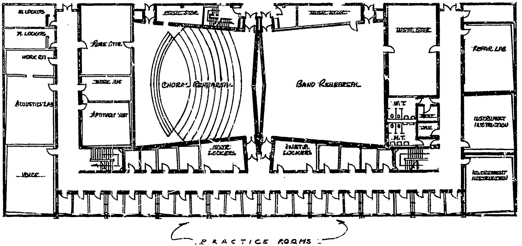
SAN FERNANDO VALLEY STATE COLLEGE - MUSIC BLDG.
