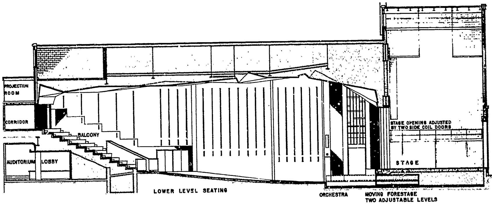
Ceiling and wall slots provide desirable front lighting. Note the two movable platforms which make possible a forestage. Evanston Township (Illinois) High School Perkins and Will, Architects
