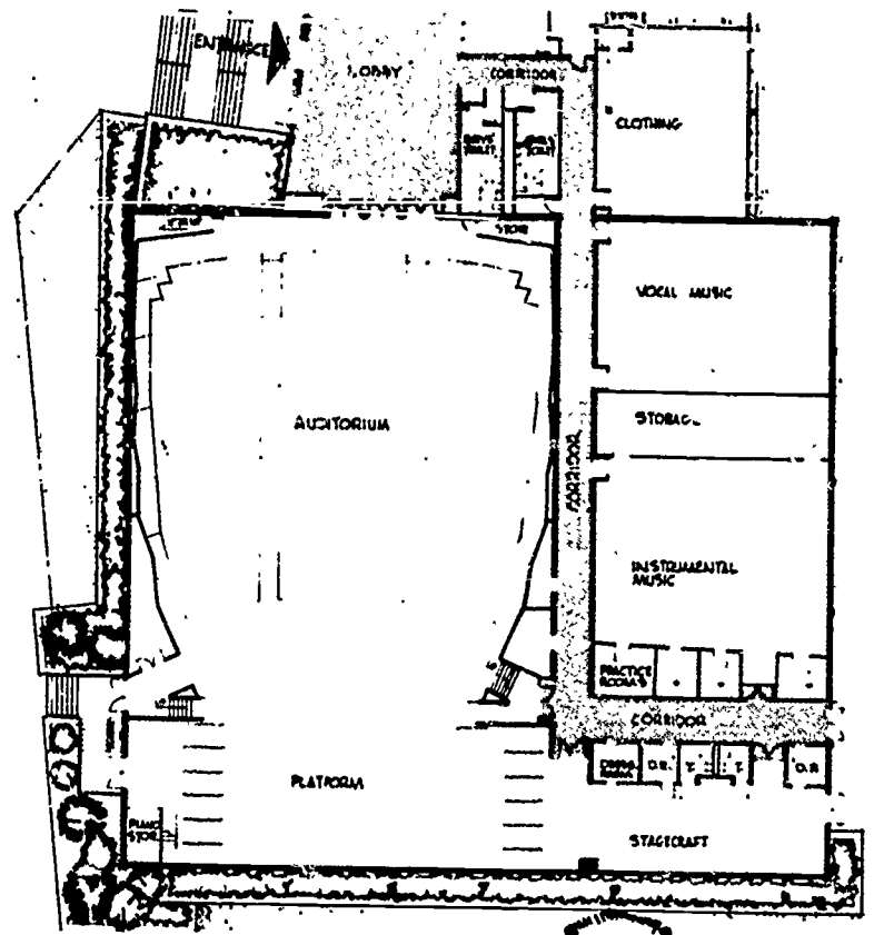
A corridor separating the music suite from the auditorium helps provide sound isolation if the doors are kept closed. Lower Merion School, Ardmore, Pennsylvania H. A. Kuljian & Company, Architects
