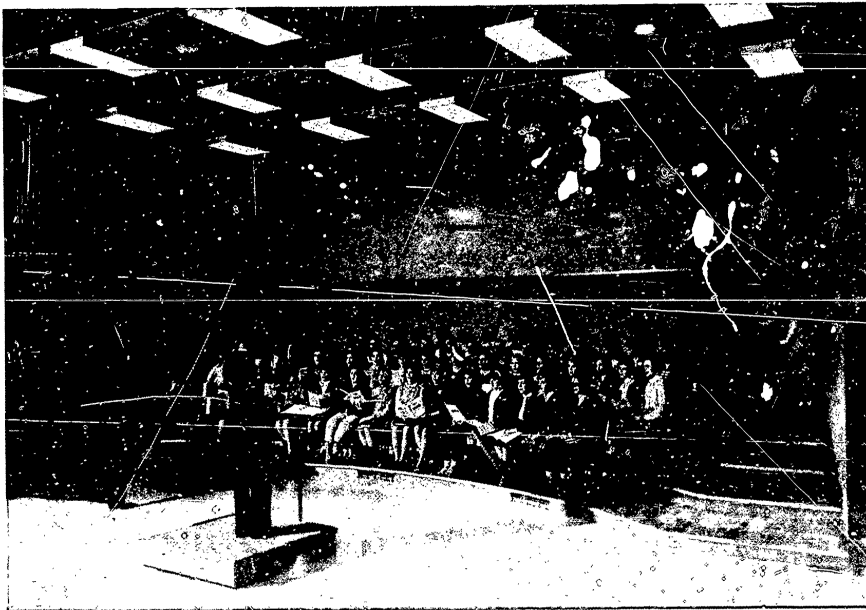
Music room activities indicate that levels in the 70 and 100 footcandle range should be used. Light colored flooring materials reduce the contrast with the printed page. Fine Arts Center, Knox College, Galesburg, Illinois Perkins & Will, Architects
