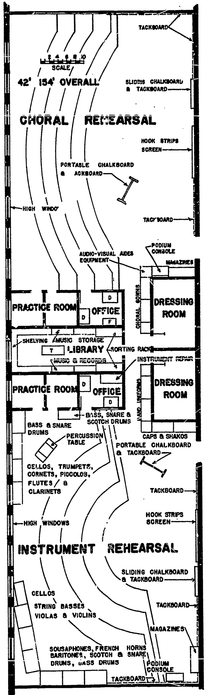
Plan for a two-teacher music department.
