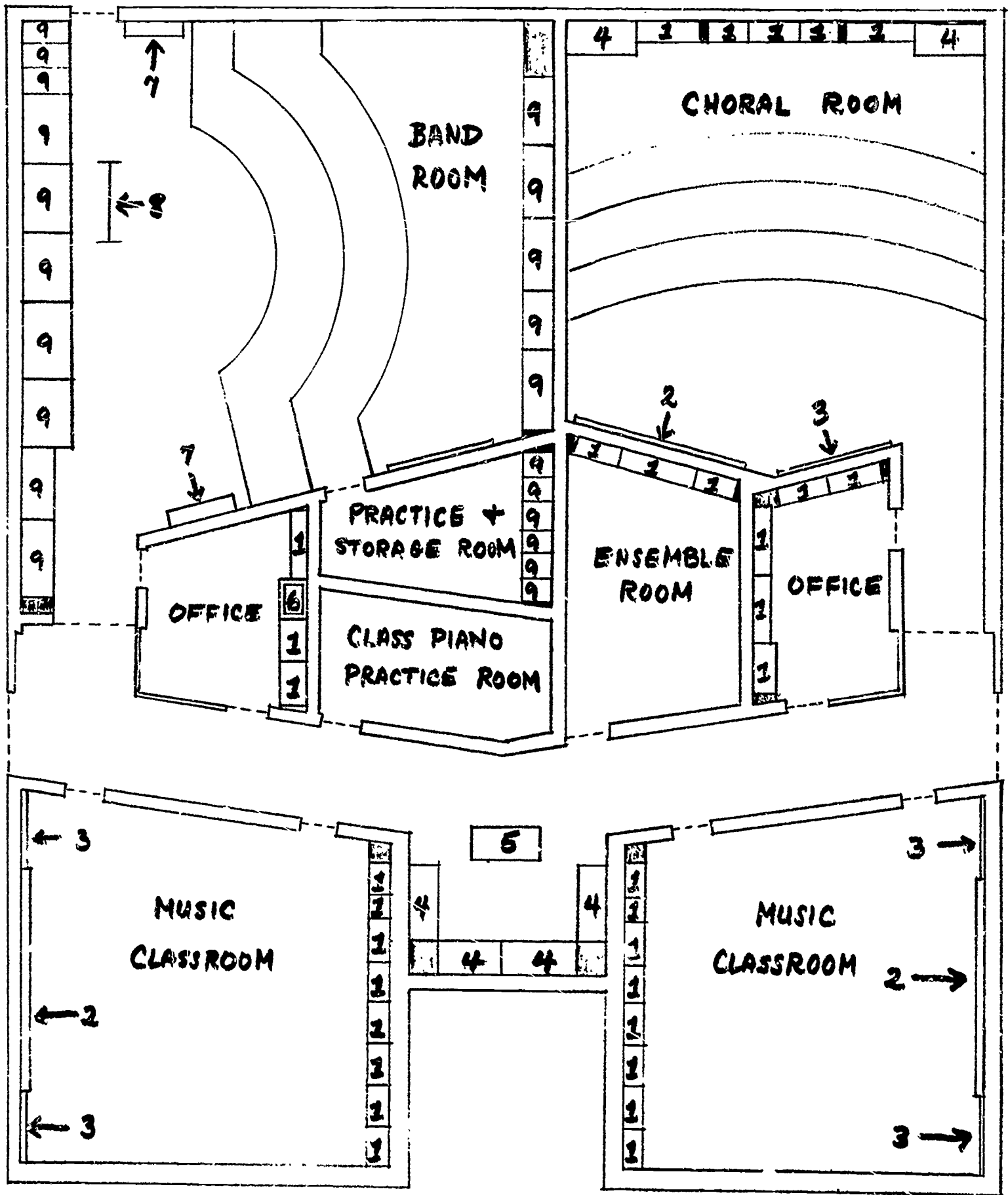
Larger practice rooms reflect the increased emphasis on small ensembles both vocal and instrumental. Governor Thomas Johnson High School, Frederick, Maryland Henry Powell Hopkins and Associates, Architects
