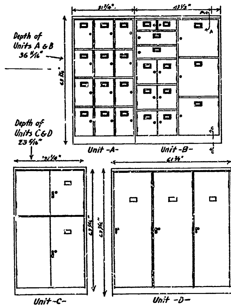
Compartments should be "tailor-made" to suit the instrumental and equipment needs. Plans from Board of Education, Pittsburgh, Pennsylvania
