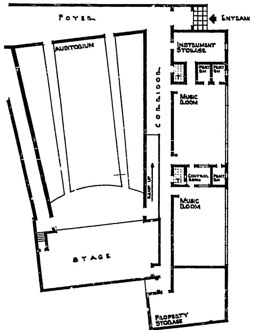
A corridor separating the music suite from the auditorium helps provide sound isolation if the doors are kept closed. Lower Merion School, Ardmore, Pennsylvania H. A. Kuljian & Company, Architects
